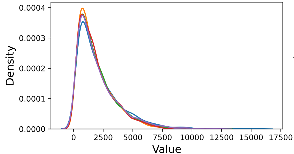
Balanced OT
